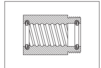
Internal Snap Ring
