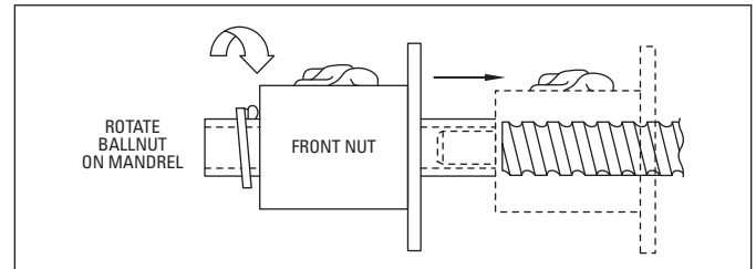
Figure 10. Transfer of front nut to screw.
