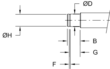
TYPE FF1, REQUIRED FOR FF SUPPORT
