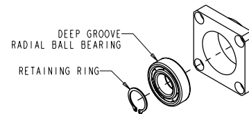
FF Bearing Support (1)(3)
