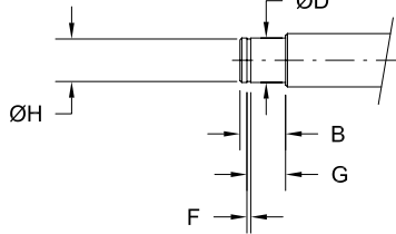
TYPE BF1, REQUIRED FOR BF SUPPORT
